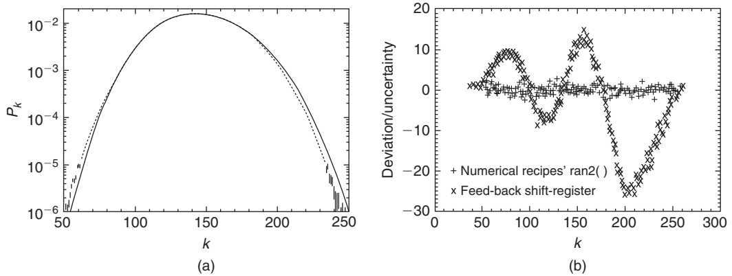
FIGURE I.1 (a) The exact energy distribution for a 32 \times 32 Ising lattice at the critical temperature (solid line) and the distribution calculated from 10^7 configurations using the Wolff Monte Carlo algorithm with the R250 feedback shift-register pseudorandom number generator (error bars). 5 The distribution calculated using the Wolff algorithm with Numerical Recipes ran2() (Press et al., 2007) is also shown, but is almost indistinguishable from the exact solid curve on this scale. (b) Deviation of the Monte Carlo results from the exact distribution in units of the statistical uncertainty of each point. The +’s indicate the ran2() results and the x’s indicate the feed-back shift-register results. The \chi^2 -value for the two cases yields \chi^2 = 190 for 210 nonzero points and \chi^2 = 2.8 \times 10^4 for 217 nonzero points, giving deviations of -0.95\sigma and 1300\sigma , respectively; see Section 13.4.A and Beale (1996).
